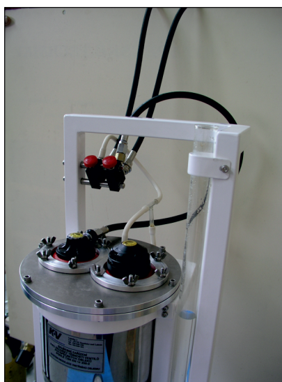
Inhalation and expiration valve – dry diver suit – cyclic tests
