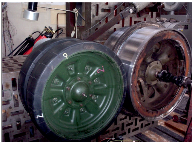
Tests of running wheels of the track vehicles
