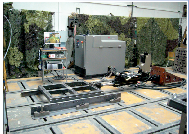
Seismic capability of nuclear power plants technologies - MTS seismic stand
