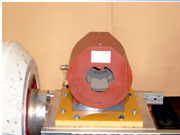
Tests of mechanical resistance of measuring transformers
