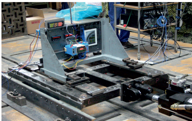
Tests of seismic capability of measuring systems
