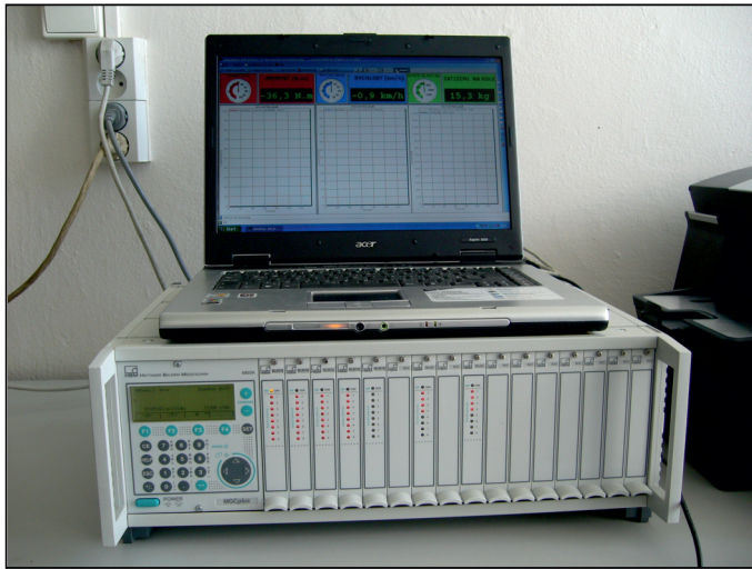
Physical quantities– 48 measuring places - HBM MGCplus measuring unit
